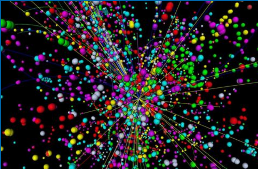
Higgs Boson particle
